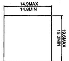
Single Panel - Latch Clearance Panel Thickness 0.062 inch
